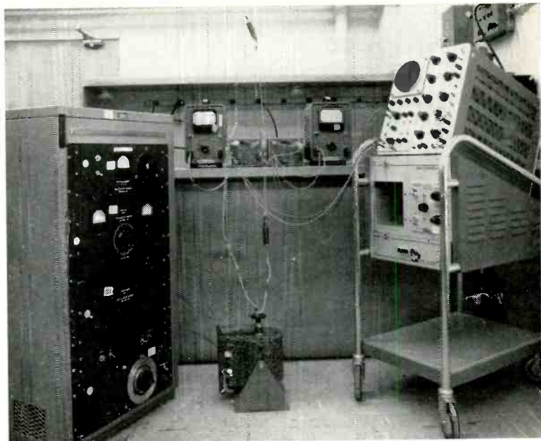
Fig. 12: Vibration exciter used for testing.
