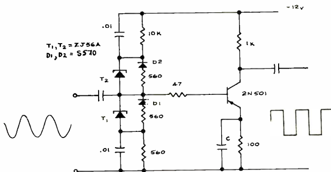
Fig. 6 (left): This flip-flop is triggered by a sine wave input.
