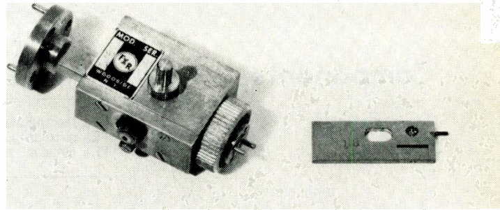
Fig. 2: The harmonic generator mount and 2mm. detector cartridge.
