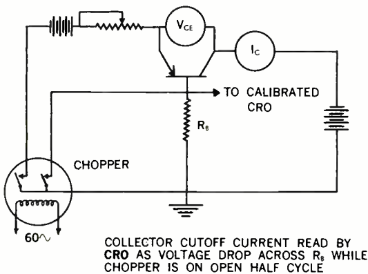
Fig. 1. Thermal resistance test
