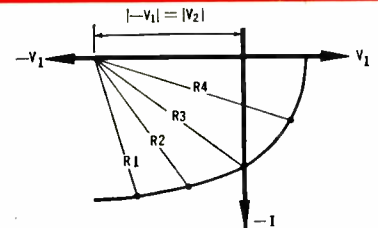
Fig. 7c: Current-voltage characteristic over silicon cell.
