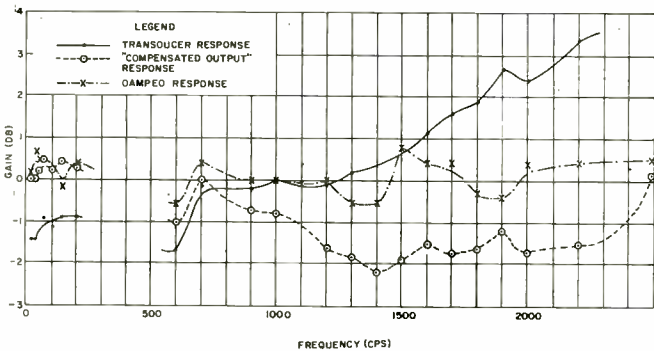
Fig. 15: Response of transducer 1. Irregularities caused by table resonances.
