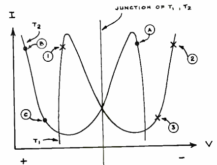
Fig. 7 (right): Curves for the circuit shown at the left, Fig. 6.
