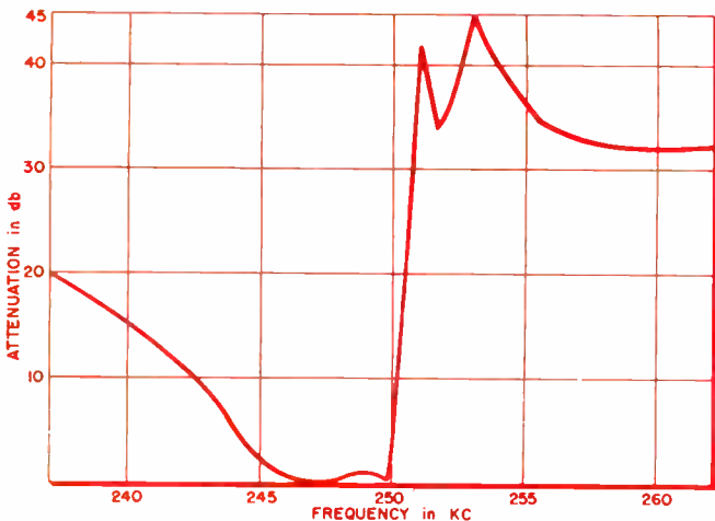
Fig. 3: Insertion-loss performance of the filter shown in Fig. 2.
