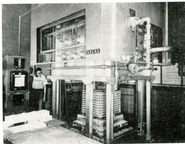
Fig. 1: Workpieces to be fired are cathode support insulators for microwave amplifier electron tubes.
