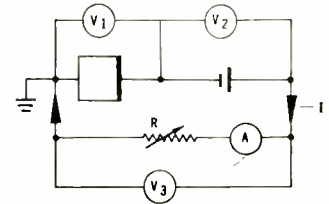
Fig. 7a: The basic circuit when photocell is operated in reverse bias condition.
