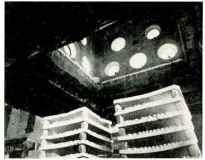
Fig. 3: Heating chamber shows pattern of the Duradiant burners in one wall.
