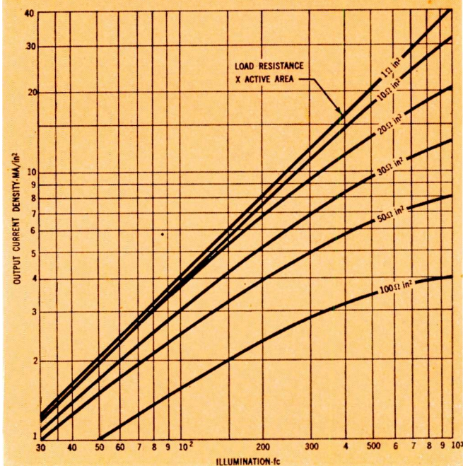
Fig. 4: Cell output current density vs. illumination intensity.
