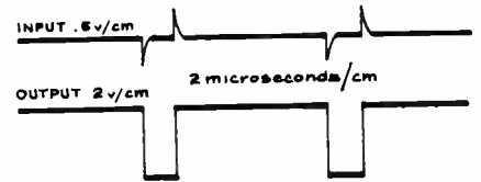
Fig. 4: The input and output waveforms for the circuit of Fig. 3.
