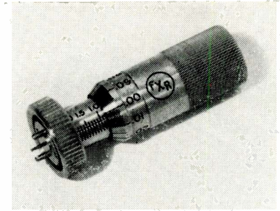
Fig. 7: The micrometer barrel of this precision sliding short has a least count of .0005 millimeter.
