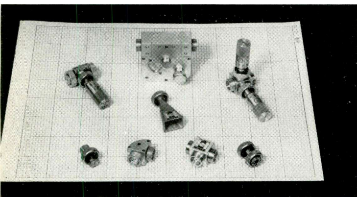
Fig. 10: Some of the components designed and tested at 2mm.
