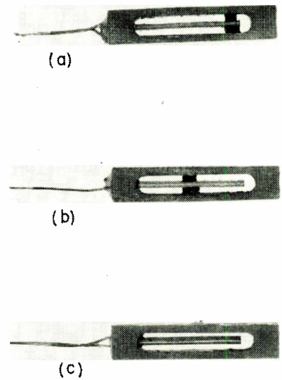
Fig. 21: (a) With Neoprene damping at free end. (b) With Neoprene damping in center; and (c) Without damping.
