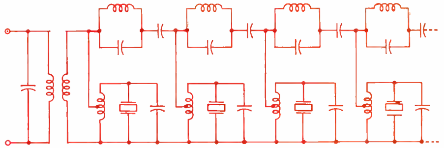
Fig. 4: Schematic of a ladder filter using quartz crystals.
