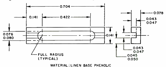
Fig. 23: One-half of transducer housing.
