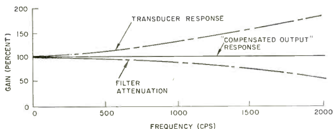
Fig. 11: "Compensated Output" derived from a combination of transducer and filter.
