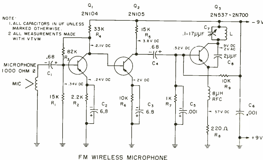
Fig. 1: Schematic diagram of the wireless mike. Oscillator tank coil is the antenna.
