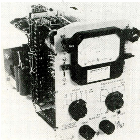
Fig. 4: Level and Gain controls are mounted alongside of meter.
