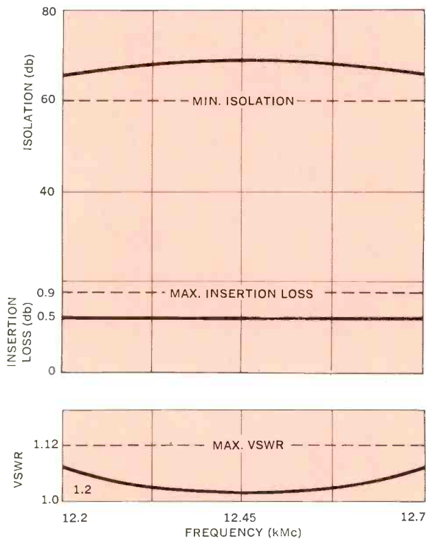
FD-7516 — TYPICAL PERFORMANCE CHARACTERISTICS (25°C)
