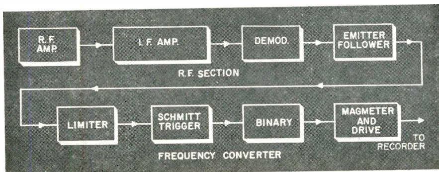
Fig. 2: Radiosonde receptor block diagram.
