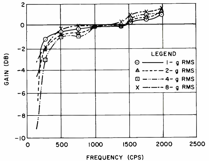
Fig. 20: Fluid damped response characteristics.
