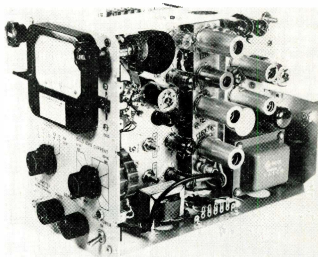
Fig. 3: Regulator amplifier is mounted in center of power meter.
