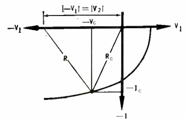
Fig. 7d: Apparent cell resistance is a function of illumination level, bias, and load resistance.
