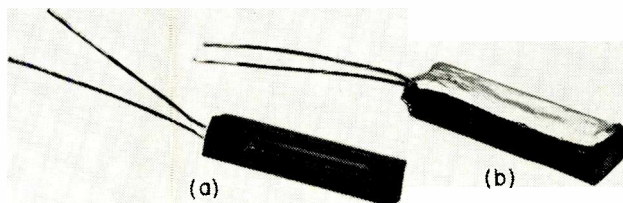
Fig. 19: Before and after damping with silicone fluid.
