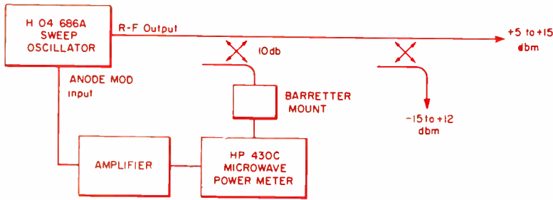
Fig. 1: Block diagram shows the microwave power regulator set-up.
