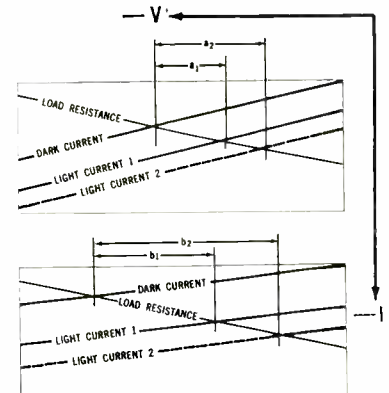
Fig. 8a & b: Graphs illustrate the effect of dark resistance and light current per unit illumination on the cell sensitivity.
