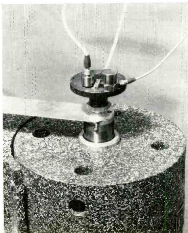
Fig. 13: Details of vibration exciter in Fig. 12.
