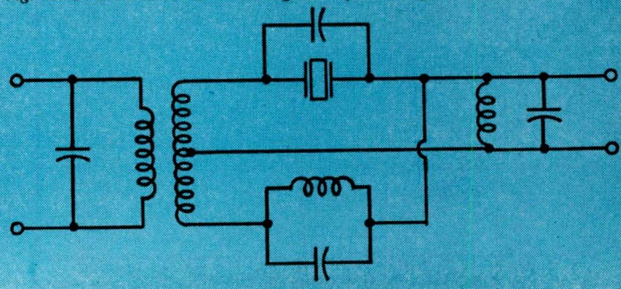
Fig. 2: Schematic of a sixth-degree crystal single sideband filter.
