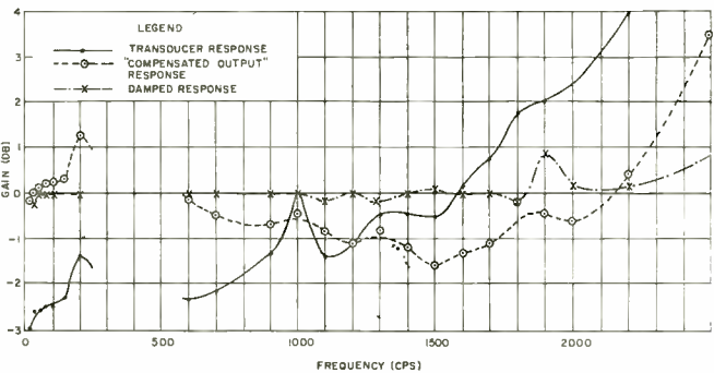
Fig. 16: Response of transducer 2. Irregularities caused by table resonances.
