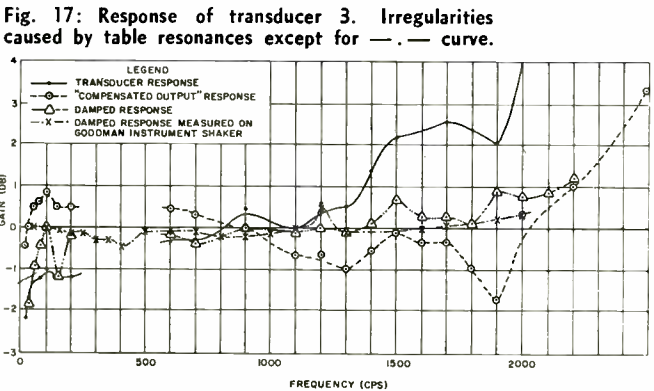
Fig. 17: Response of transducer 3. Irregularities caused by table resonances except for — — curve.
