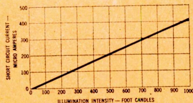
Fig. 2: Short circuit current vs. illumination intensity for readout cell.
