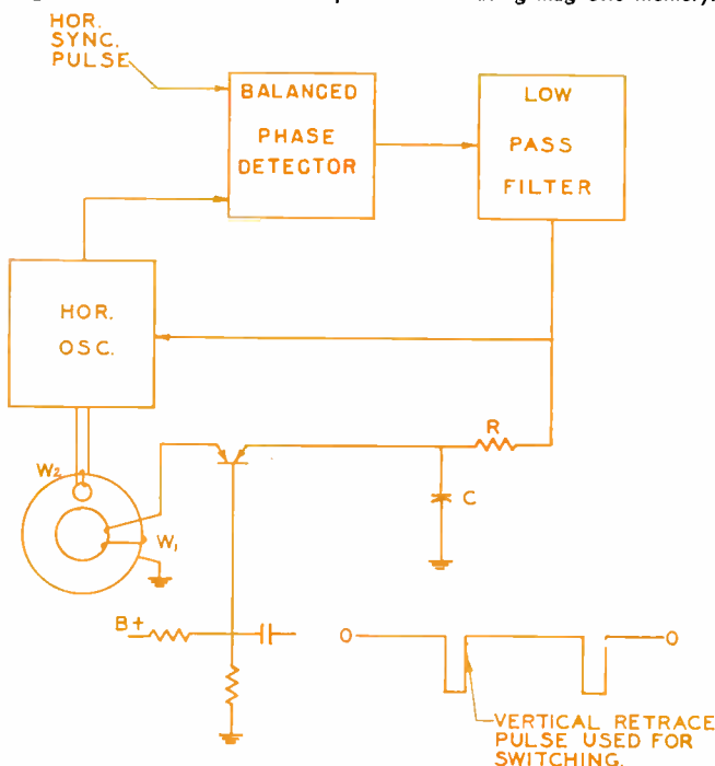
Fig. 6: Horizontal TV oscillator phase control using magnetic memory.
