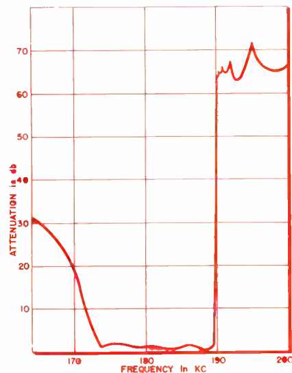
Fig. 5: Insertion-loss performance of the filter circuit of Fig. 4.
