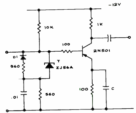
Fig. 5: An improved version of the circuit shown in Fig. 3.
