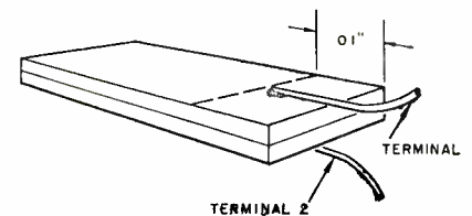
Fig. 22: Terminal leads soldered to crystal.
