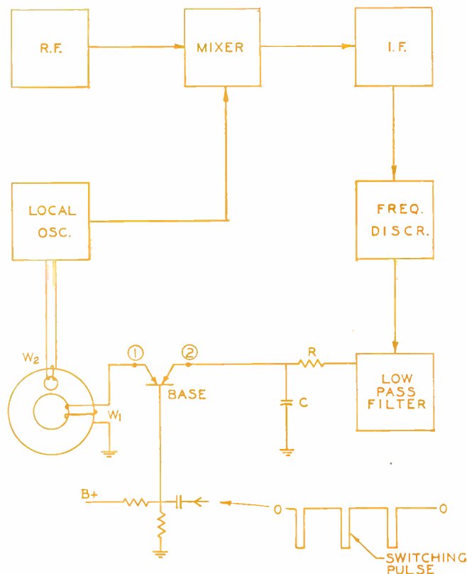
Fig. 4: AFC system with magnetic memory and transistor switch.
