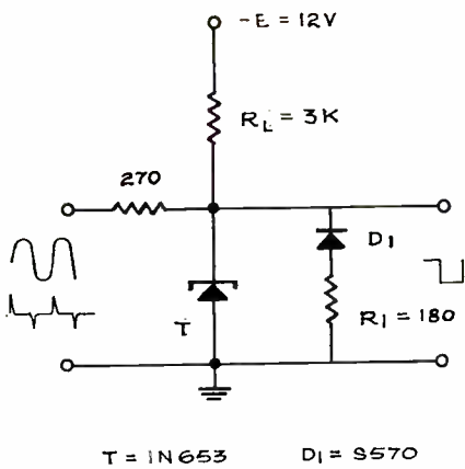
Fig. 2 (left): A gallium arsenide tunnel diode is used in this constant current flip-flop circuit.
