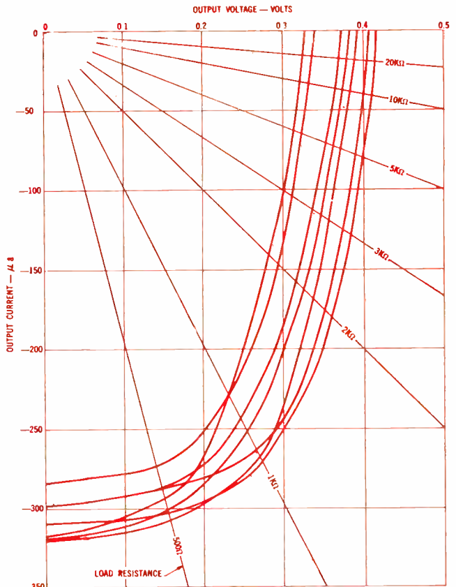
Fig. 6: With light intensity of 600 footcandles, the normal spread in output characteristics for cell modules is shown.
