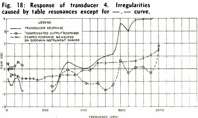
Fig. 18: Response of transducer 4. Irregularities caused by table resonances except for — — curve.
