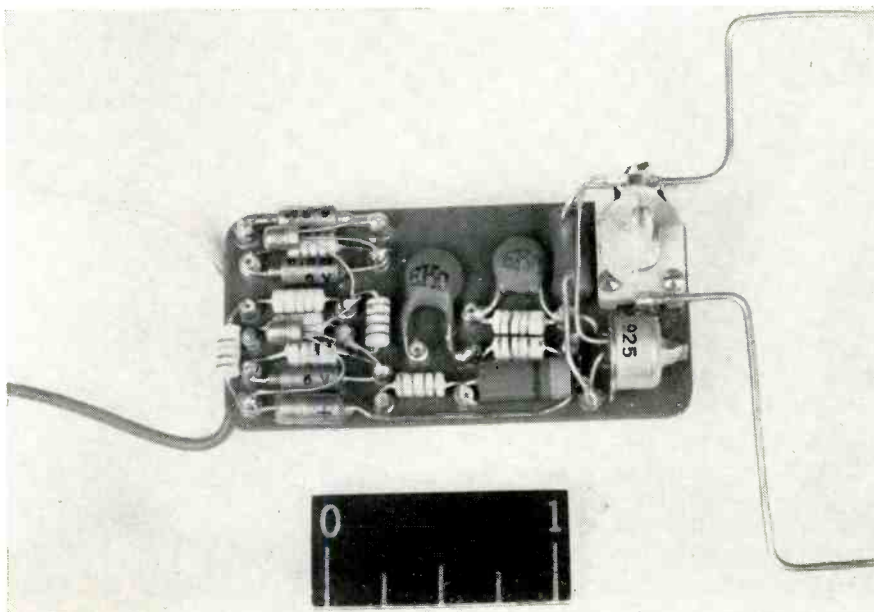
Fig. 6: Photograph shows parts layout for circuit in Fig. 5 above.
