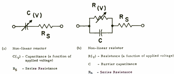
Fig. 1: Simplified equivalent circuit for (a) the non-linear reactor and (b) the non-linear resistor crystal harmonic generators.
