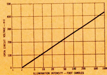
Fig. 3: Open circuit voltage is plotted against illumination intensity.
