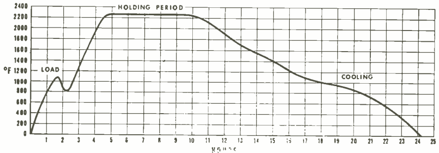
Fig. 4: Heating operation.
