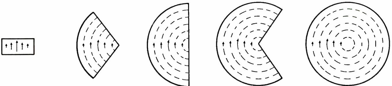
Fig. 3: Transition from the TE 10 rectangular to the TE 01 circular waveguide mode.
