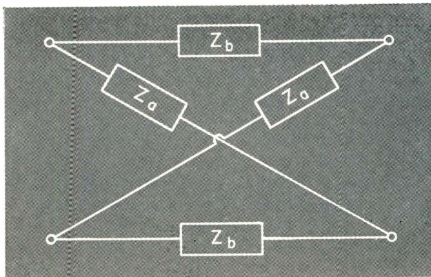
Fig. 1: The lattice circuit and its equivalents are the most widely used configurations for the realization of crystal filters.
