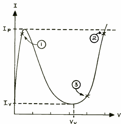
Fig. 1: The well known characteristic curve of the tunnel diode.
