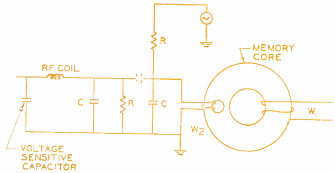
Fig. 7: Circuit for using an inductance memory at very high frequency.
