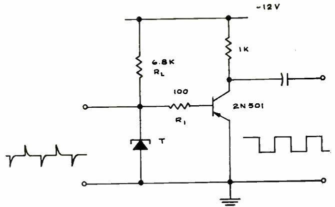
Fig. 3 (right): Constant current flip-flop and amplifier circuit.
