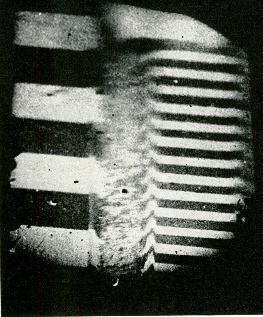
Photomicrograph of magnetically recorded pattern, taken with polarized light, compares readout capability of present systems (left) and NCR MAGOP unit (right).
