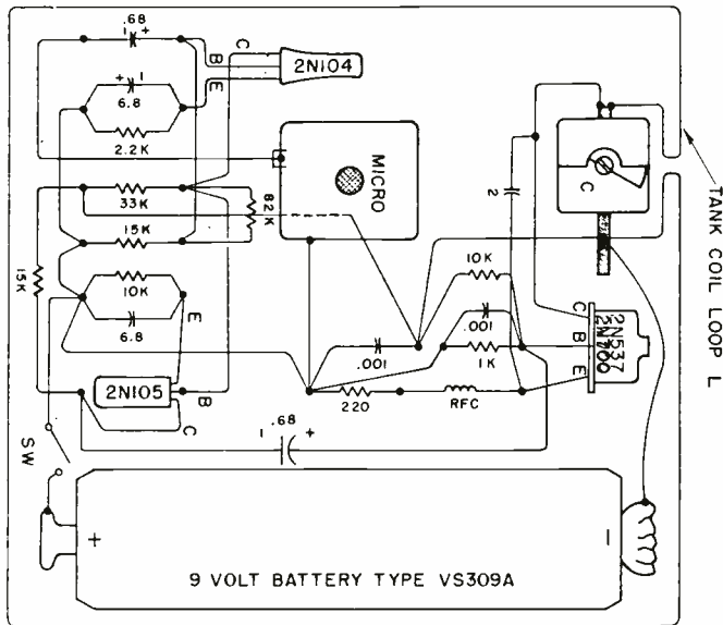
Fig. 2 (left): Wiring diagram of wireless mike shows the general layout of parts.
