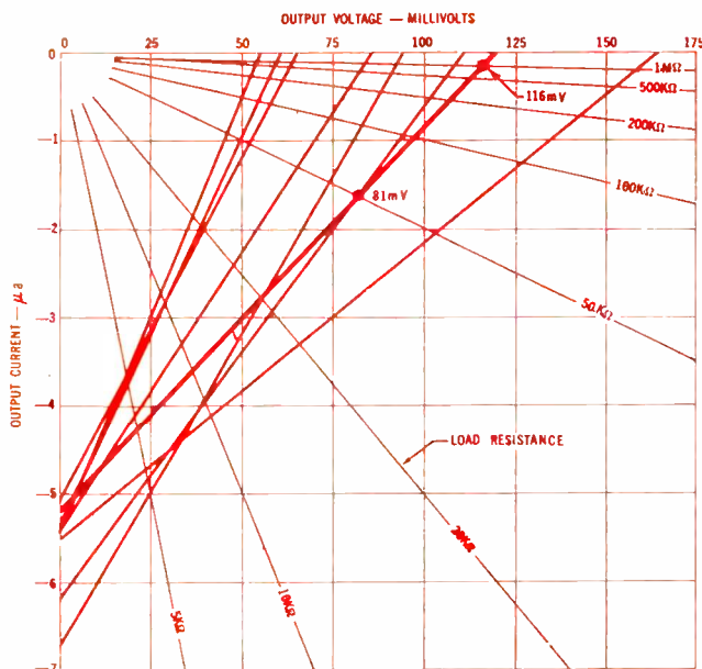
Fig. 5: The normal spread in output characteristics for cell modules is shown for light intensity of 15 footcandles.
