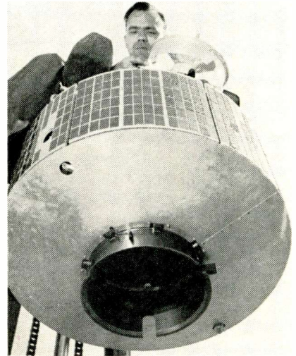
Communications satellite developed by Hughes Aircraft Co. can handle hundreds of telephone circuits and direct TV transmission if placed in equatorial orbit at 22,000 mi. altitude. James C. Meyer, environmental engineer, inspects the device's 2,700 power providing, solar cells.
