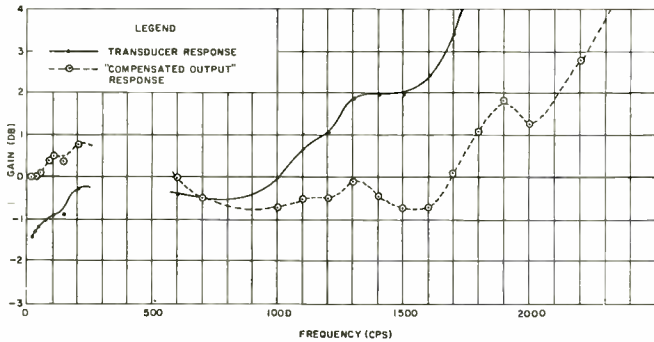
Fig. 14: Comparison of "compensated output" with normal response. Note: irregularities were caused by table resonances.
