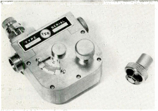
Fig. 9: Slotted section and the fixed short, showing the precision milled block construction of the unit.
