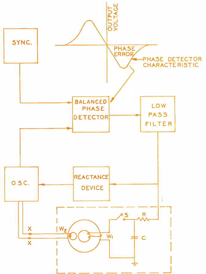
Fig. 5: Automatic phase control system with magnetic memory.
